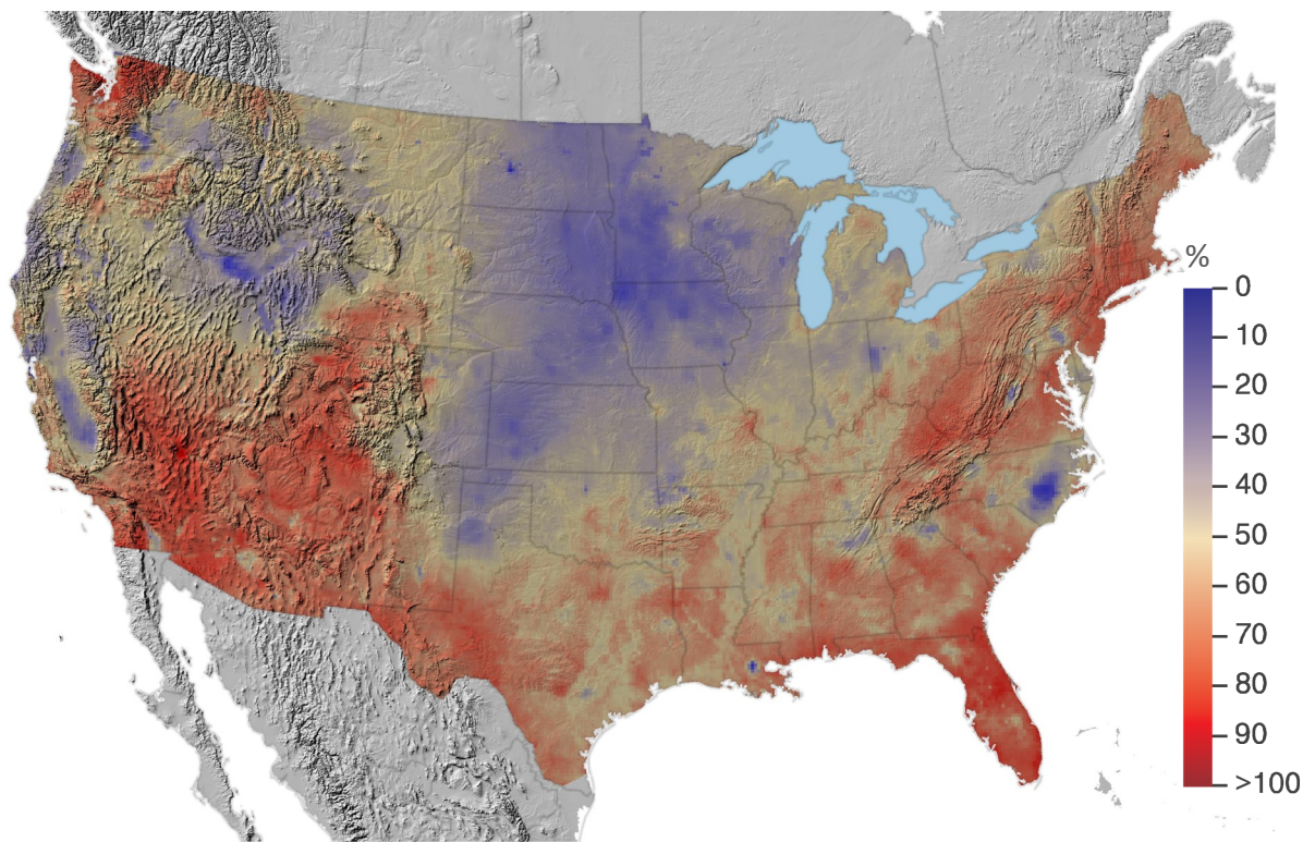
Annual oxidized nitrogen deposition in 2017 (top), and percentage of total nitrogen deposition as oxidized nitrogen in 2017 (bottom)
