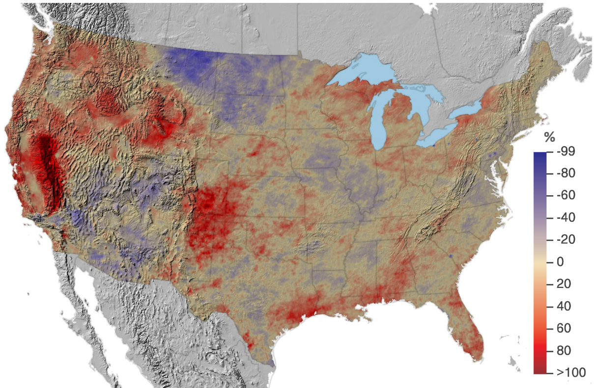
Total annual precipitation in 2017 (top), and percent deviation of 2017 precipitation values compared to the annual average of 2000-2017 (bottom)
