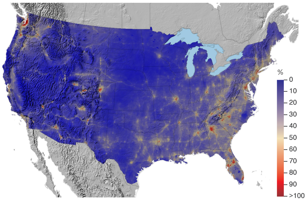
Annual deposition of unmonitored nitrogen compounds in 2017 (top), and percentage of total nitrogen deposition as unmonitored nitrogen compounds (bottom).
