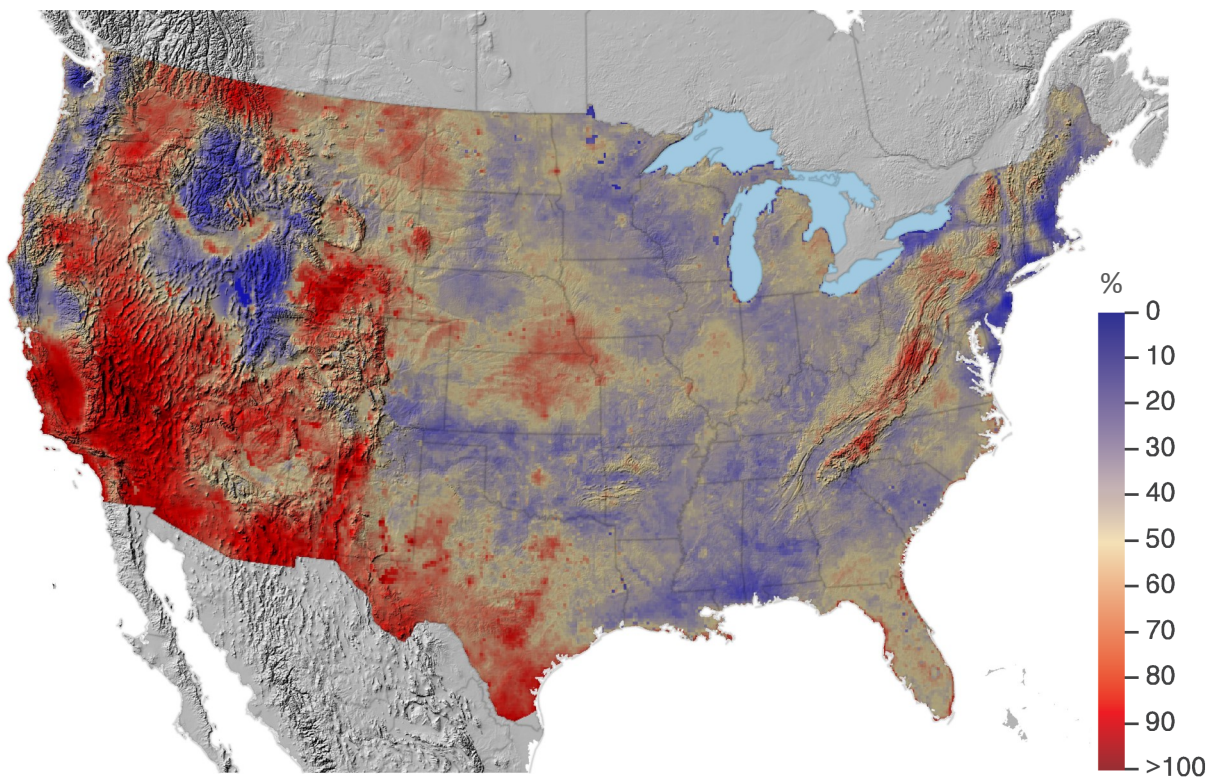
Annual base cation deposition in 2017 (top), and percentage of total base cation deposition as dry deposition in 2017 (bottom)
