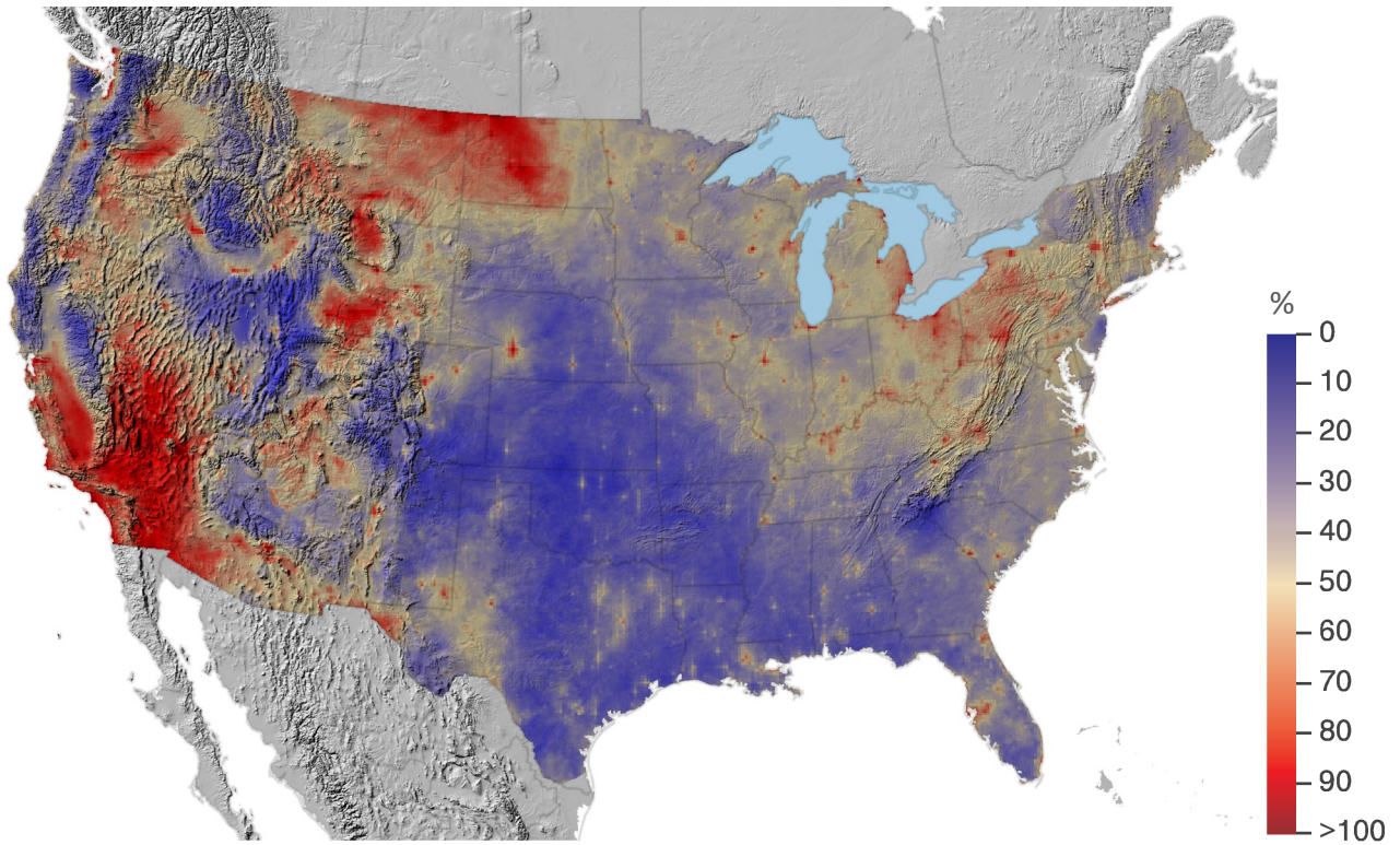
Annual sulfur deposition in 2017 (top), and percentage of total sulfur deposition as dry deposition in 2017 (bottom)
