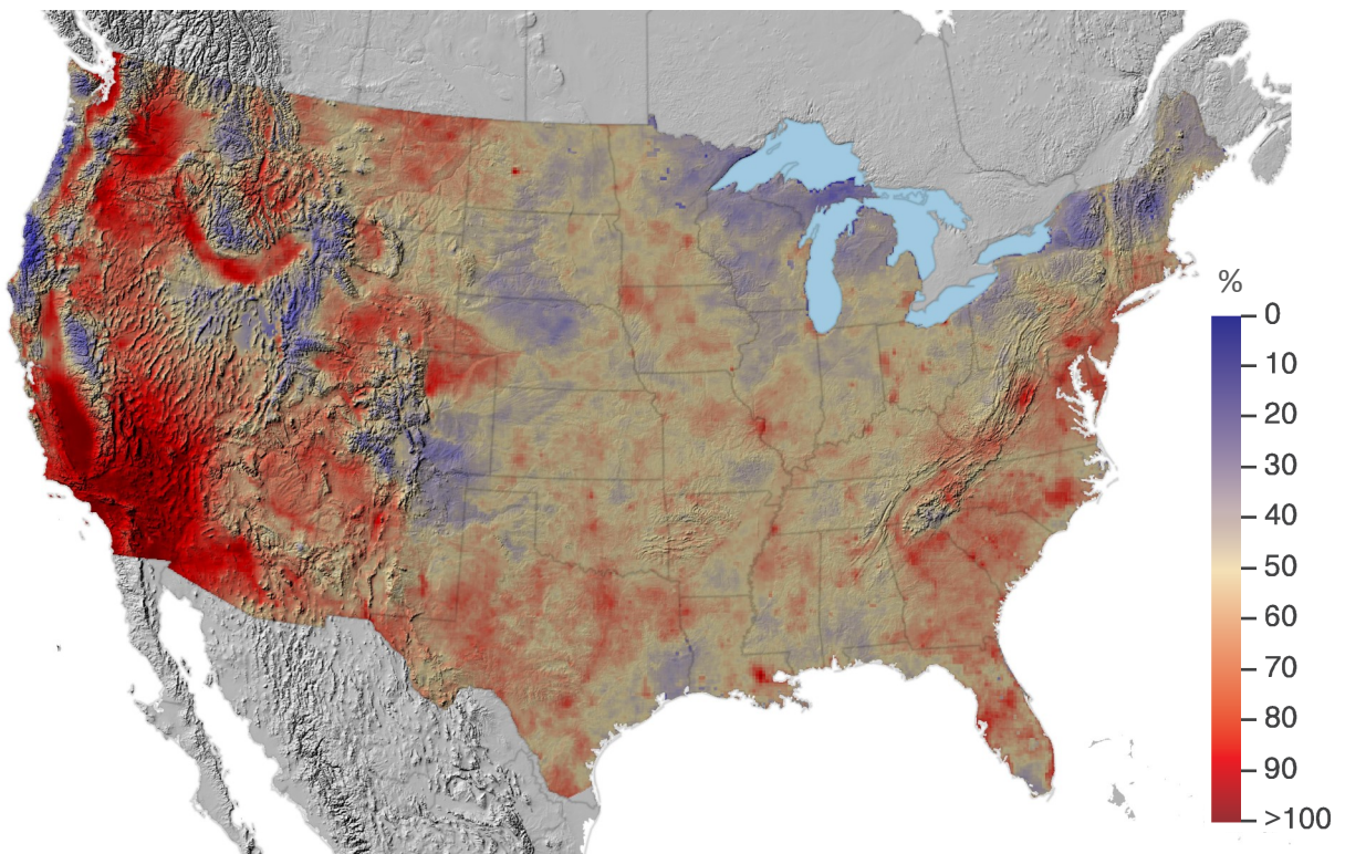
Annual dry nitrogen deposition in 2017 (top), and percent of total nitrogen deposition as dry deposition in 2017 (bottom)
