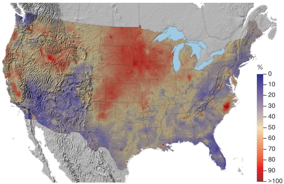
Annual reduced nitrogen deposition in 2017 (top), and percentage of total nitrogen deposition as reduced nitrogen in 2017 (bottom)
