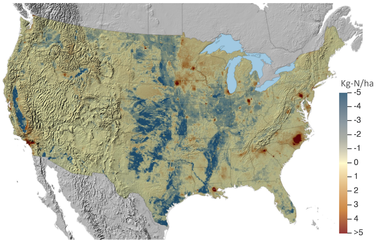
Annual gross ammonia deposition in 2017 (top), and net ammonia deposition in 2017 (bottom)
