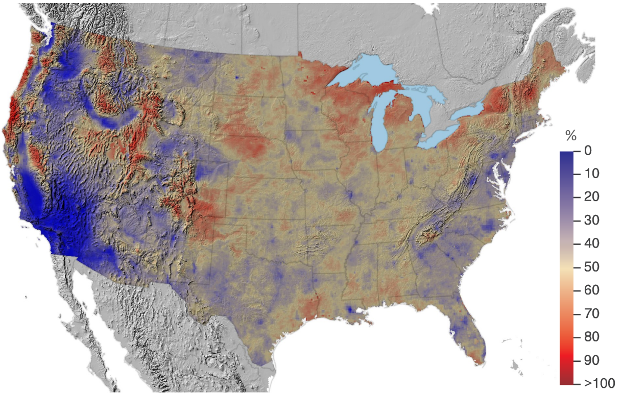
Annual wet nitrogen deposition in 2017 (top), and percent of total nitrogen deposition as wet deposition in 2017 (bottom)
