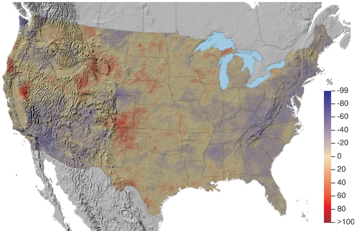
Total nitrogen deposition in 2017 (top), and percent deviation of 2017 nitrogen deposition values compared to the annual average of 2000-2017 (bottom)
