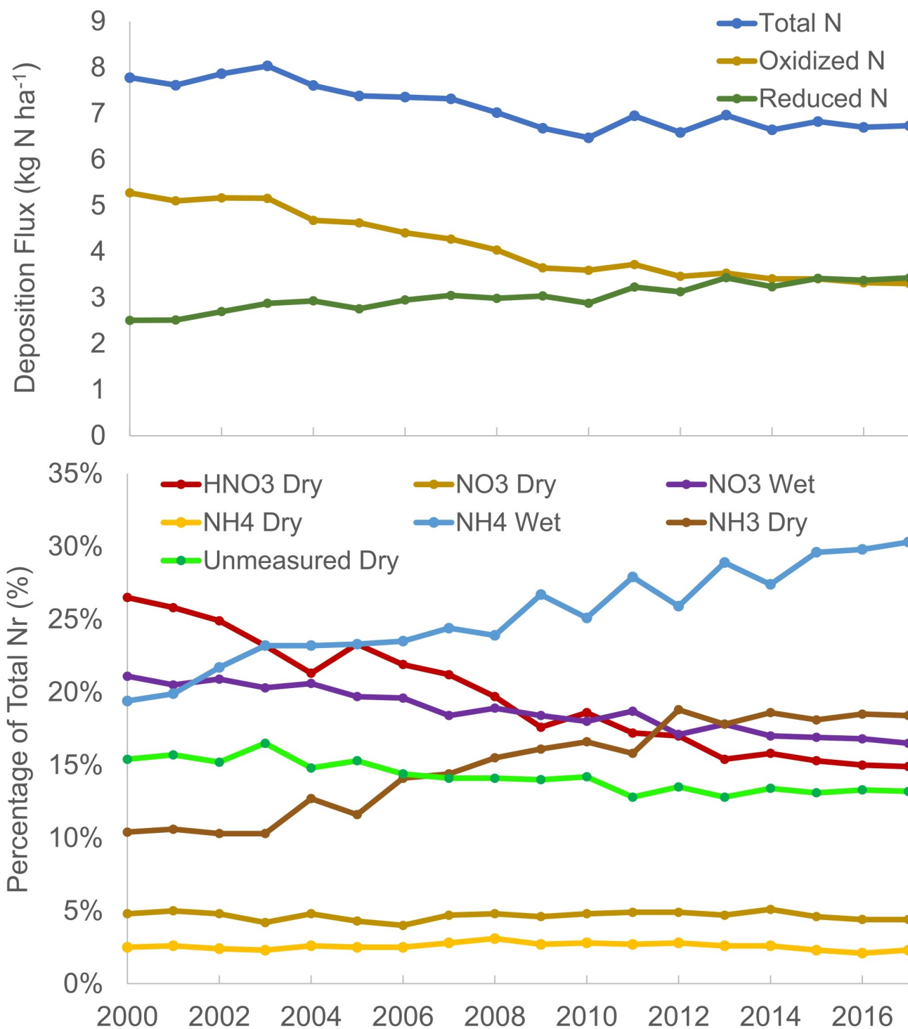
Time-series plots of annual deposition fluxes averaged over all grid cells for total N, oxidized N species, and reduced N species (top plot). Average annual deposition over all grid cells for each N species as a percentage of the average annual total N deposition flux (bottom plot).
