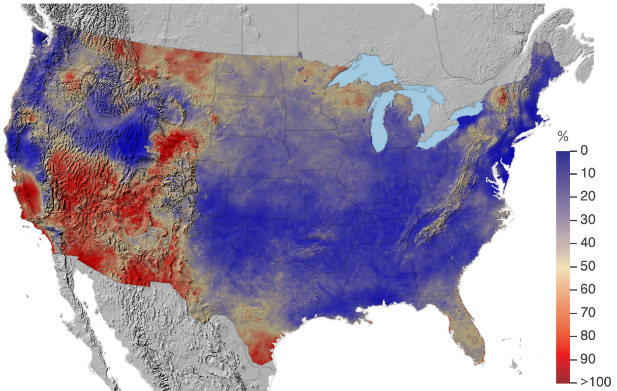
Annual chloride deposition in 2017 (top), and percentage of total chloride deposition as dry deposition in 2017 (bottom)
