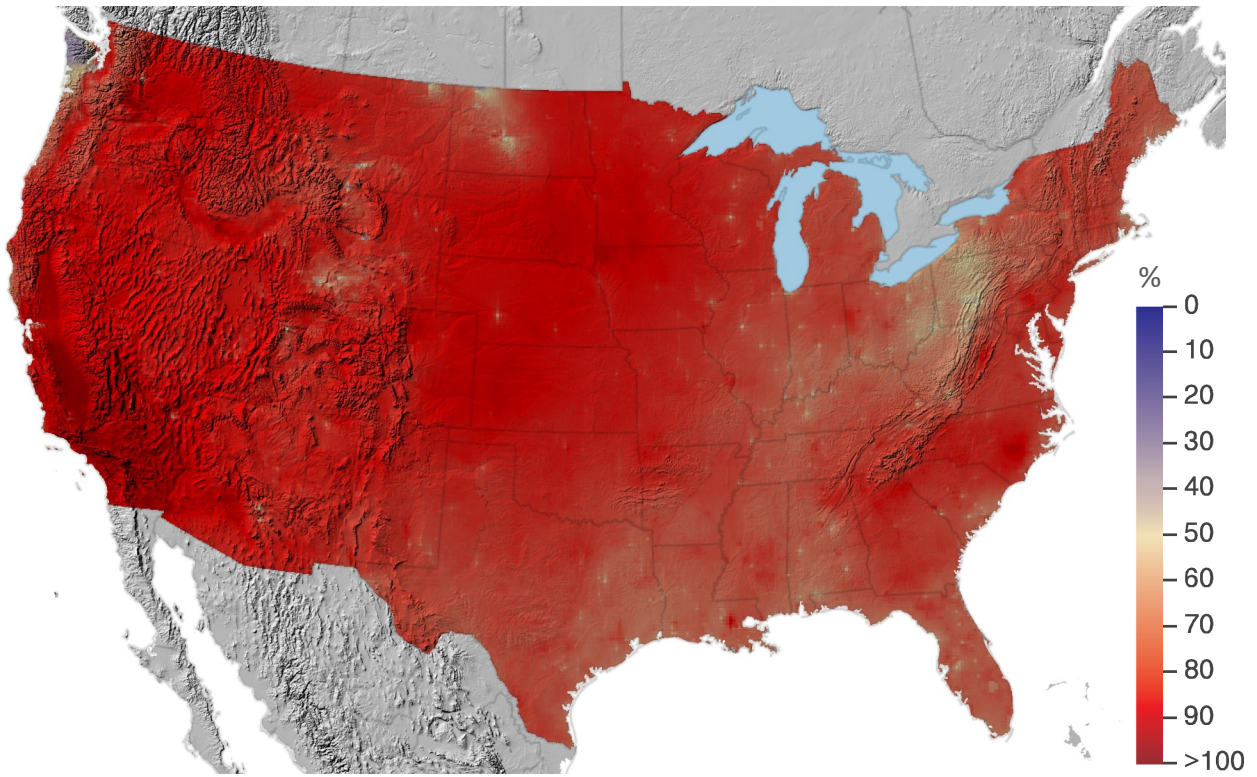
Annual S+N equivalent deposition in 2017 (top), and the percentage of S+N equivalent deposition as nitrogen in 2017 (bottom).
