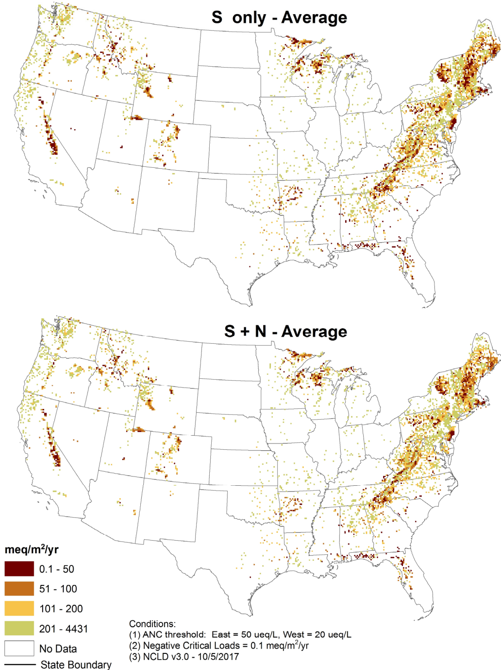
Surface Water Critical Loads for Acidity. Average aggregation for 12 x 12 km grid cell with S only (top) and S + N only (bottom) (See Lynch et al. (2017) for data source information).
