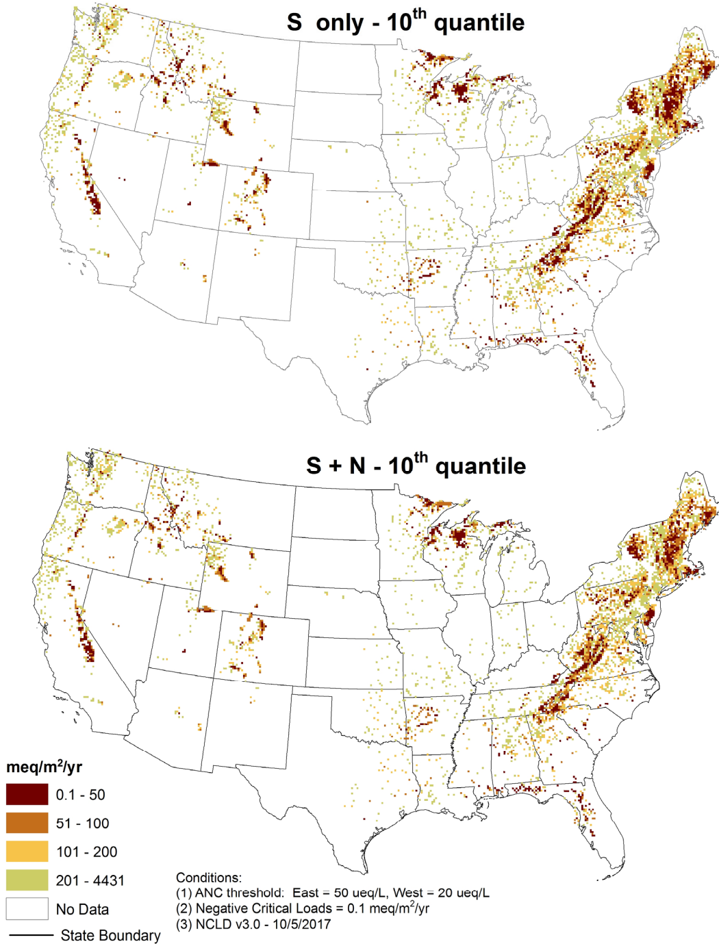
Surface Water Critical Loads for Acidity. 10 th quantile aggregation for 12 x 12 km grid cell with S only (top) and S + N (bottom) (See Lynch et al. (2017) for data source information).
